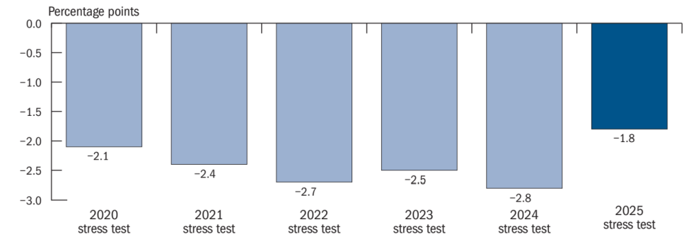
Figure 2. Aggregate maximum decline in stressed common equity tier 1 capital ratio, severely adverse scenario
